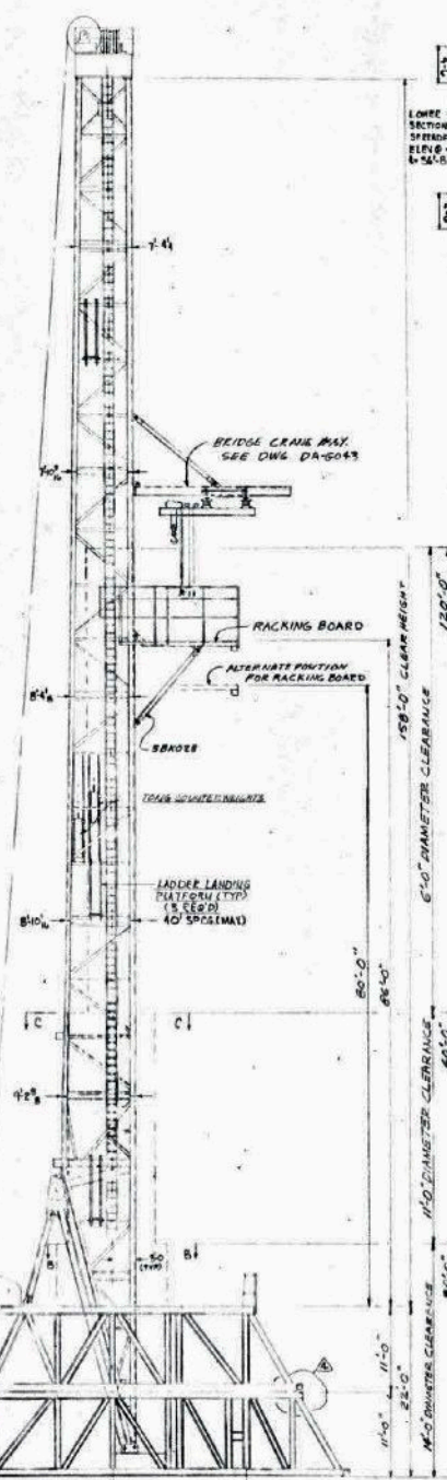
ELEVATION - MILLERS SIDE
