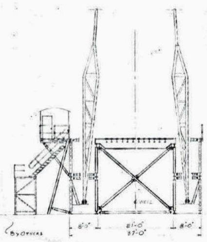
ELEVATION - V-DOOR SIDE
